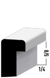
280 Back Band 11/16 x 1-1/8 PRIMED 16'
