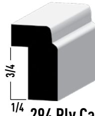
294 Ply Cap 21/32 x 1-3/32 PINE RL
