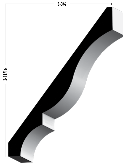
L 46 9/16 x 5-1/4 PRIMED 16'
