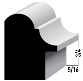
L CAP EC 1-3/8 x 1-3/4 PRIMED 16'
